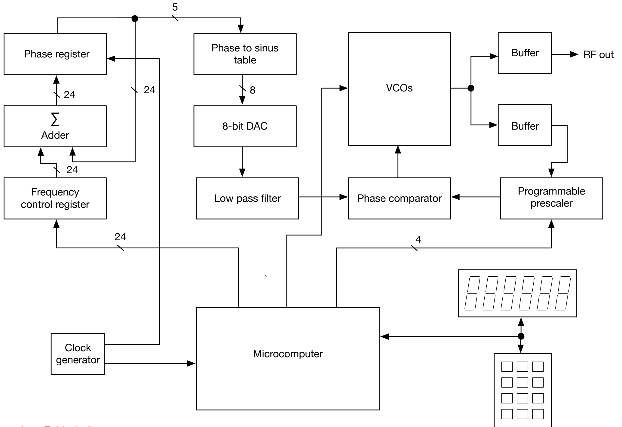
L412Z, block diagram
